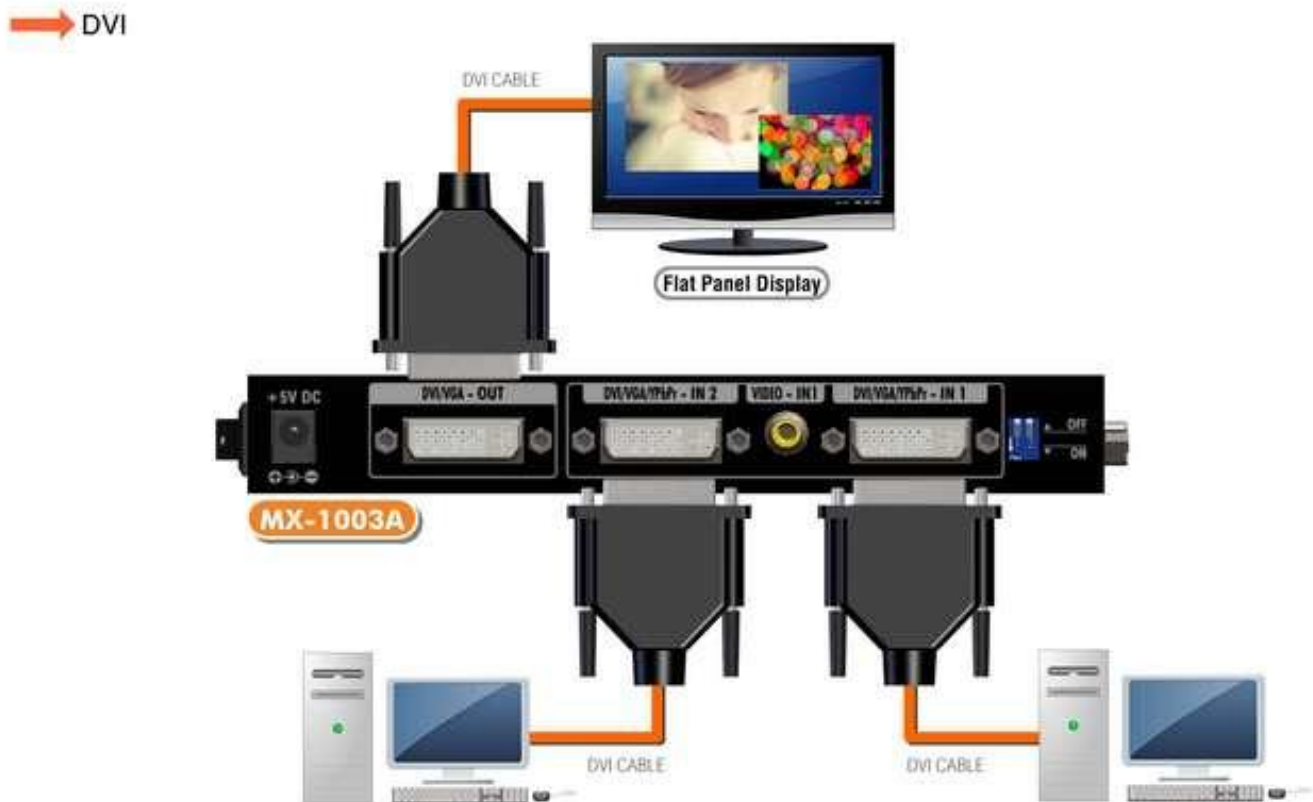
Figure 1: Configuration Diagram
