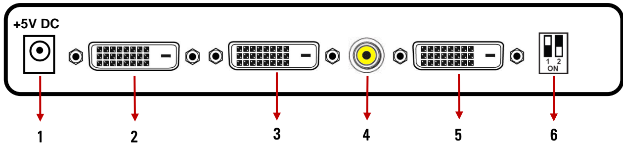
Figure 2: Rear Panel
